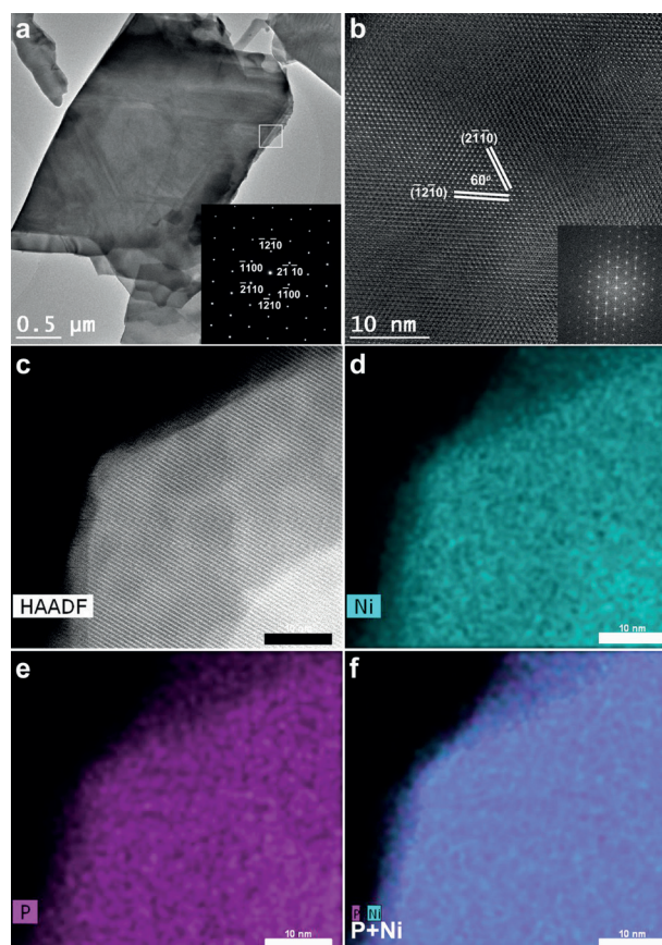
Figure 3. a) TEM and b) HRTEM images of a single NS. Corresponding SAED and FFT-ED patterns are shown as insets. c) HAADF-STEM image together with elemental maps for d) Ni, e) P, and f) P + Ni. Scale bars in c–f: 10 nm.
